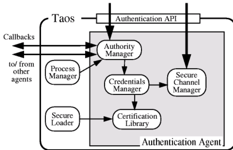
Figure 2: Structure of the authentication agent
